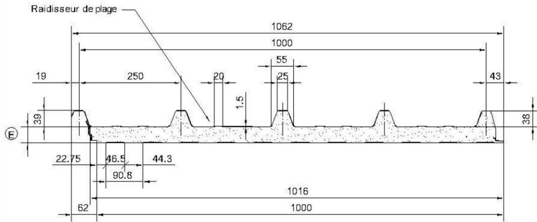
Figure 1 - Coupe transversale
